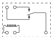
接线图(底视图) Wiring Diagram (Bottom View)
