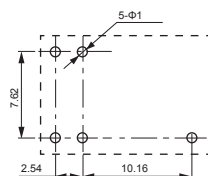
安装孔位图(底视图) Mounting Hole Layout (Bottom View)
