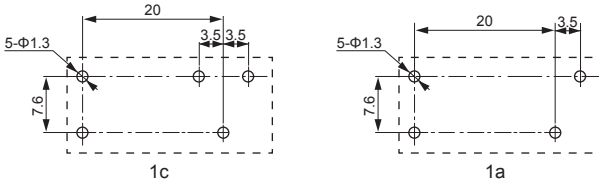
安装孔位图(底视图) Mounting Hole Layout (Bottom View)
