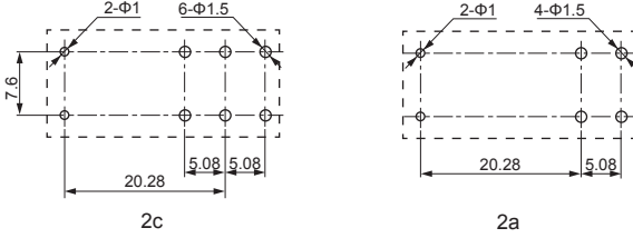
安装孔位图(底视图) Mounting Hole Layout (Bottom View)
