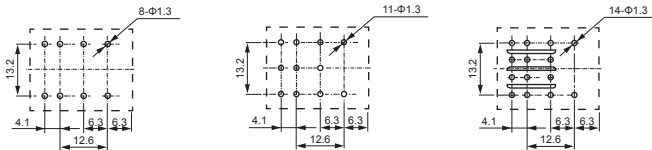
安装孔位图(底视图) Mounting Hole Layout (Bottom View)
