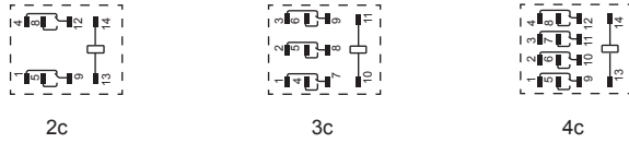
接线图(底视图) Wiring Diagram (Bottom View)
